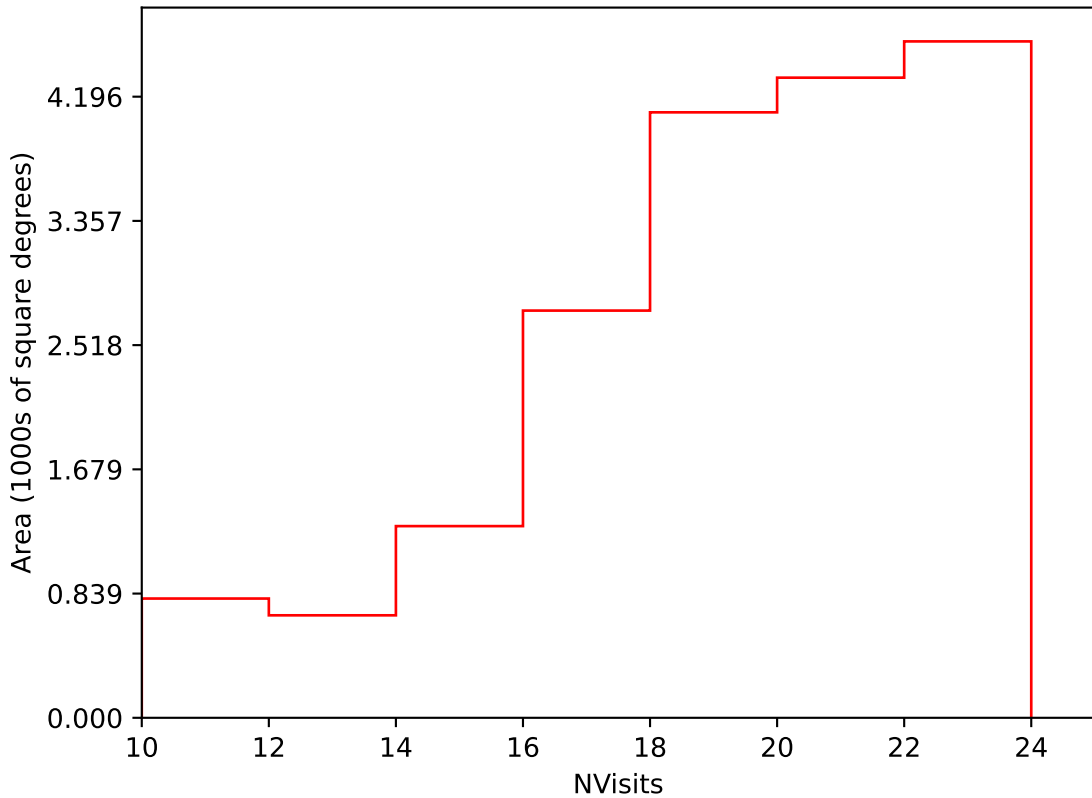
too_elab_r128_d3_ugrizy_v3.4_10yrs Yr 1 i band: NVisits
