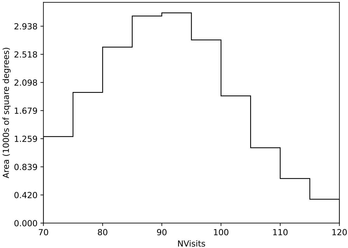
too_elab_r128_d3_ugrizy_v3.4_10yrs Yr 1 all bands: NVisits
