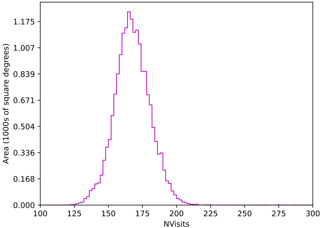
too_elab_r128_d3_ugrizy_v3.4_10yrs WFD z band: NVisits
