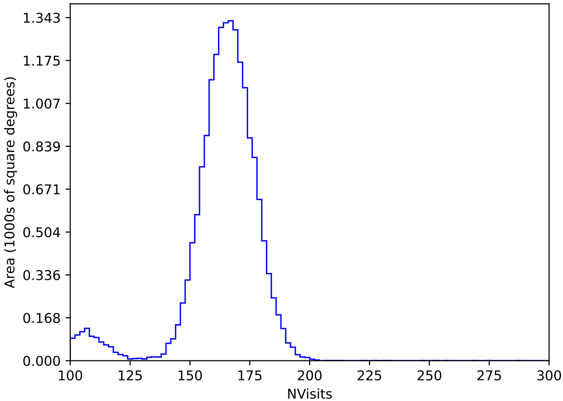
too_elab_r128_d3_ugrizy_v3.4_10yrs WFD y band: NVisits
