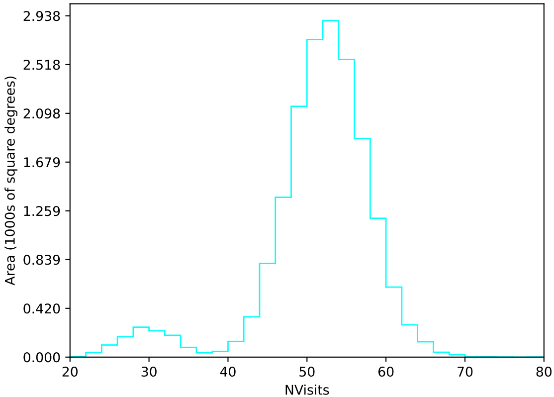
too_elab_r128_d3_ugrizy_v3.4_10yrs WFD u band: NVisits
