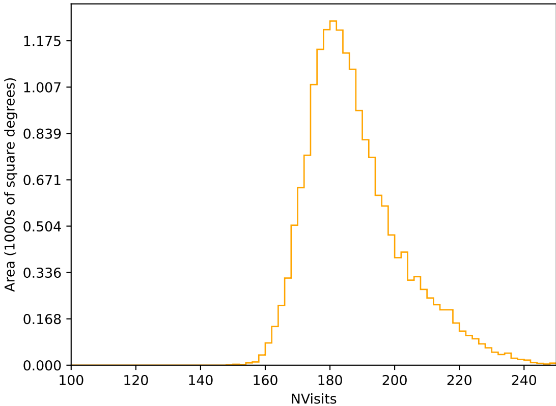
too_elab_r128_d3_ugrizy_v3.4_10yrs WFD r band: NVisits
