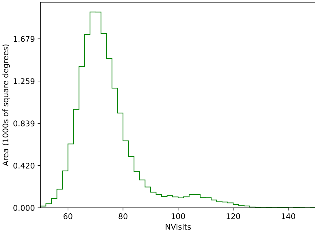
too_elab_r128_d3_ugrizy_v3.4_10yrs WFD g band: NVisits
