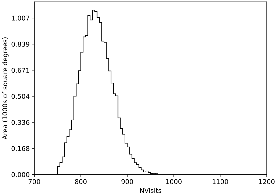
too_elab_r128_d3_ugrizy_v3.4_10yrs WFD all bands: NVisits
