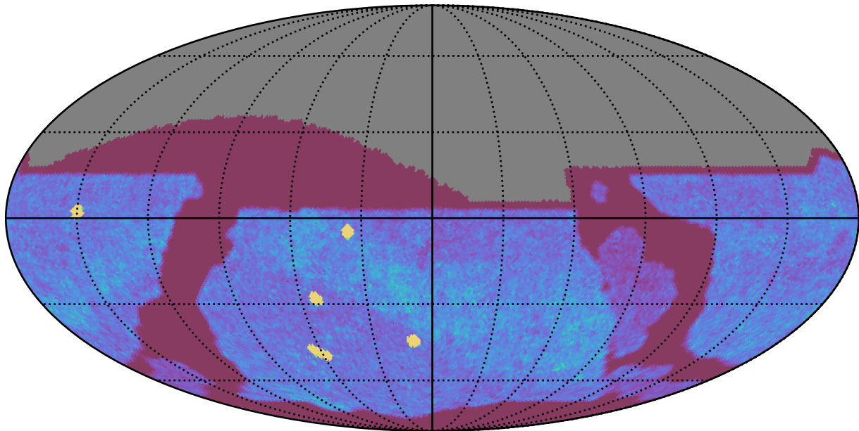
too_elab_r128_d3_ugrizy_v3.4_10yrs All sky z band: NVisits
