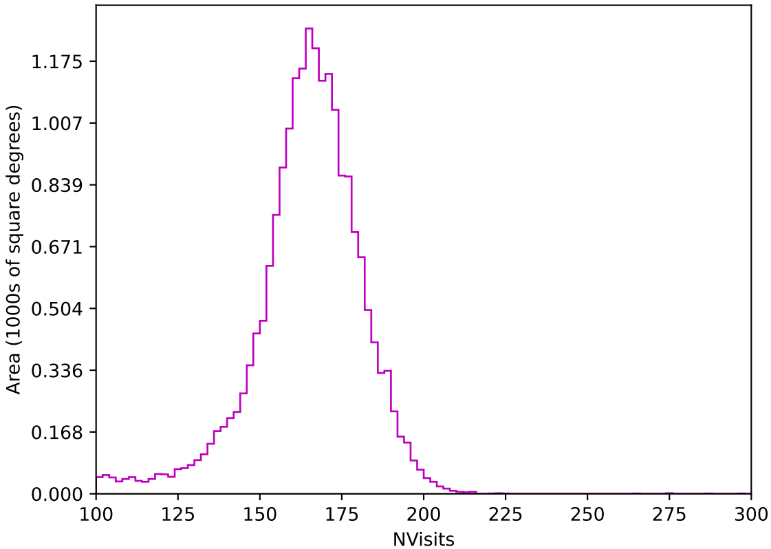
too_elab_r128_d3_ugrizy_v3.4_10yrs All sky z band: NVisits
