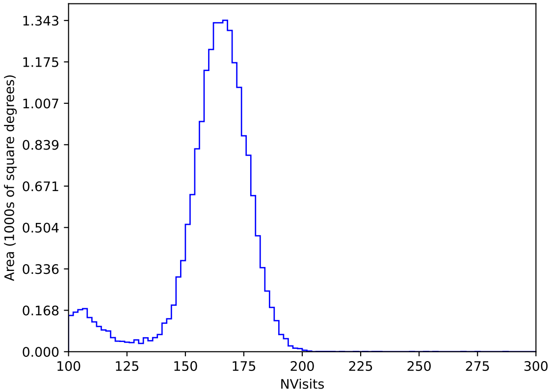
too_elab_r128_d3_ugrizy_v3.4_10yrs All sky y band: NVisits
