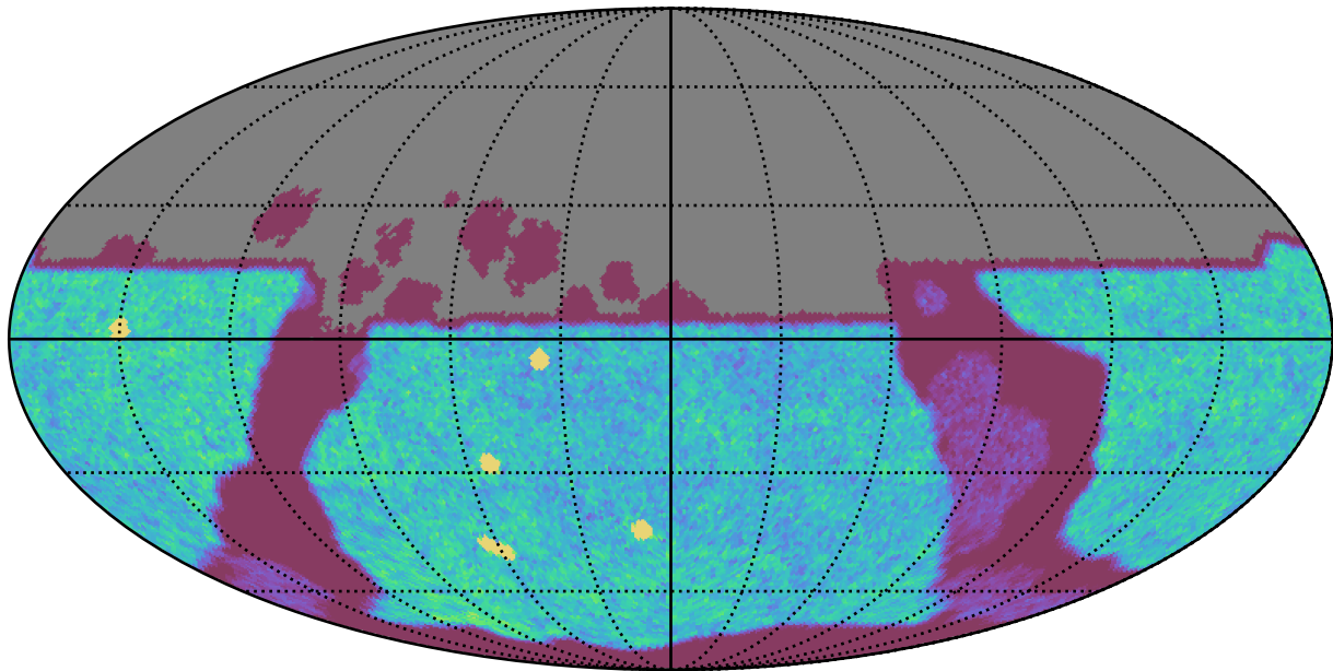
too_elab_r128_d3_ugrizy_v3.4_10yrs All sky u band: NVisits
