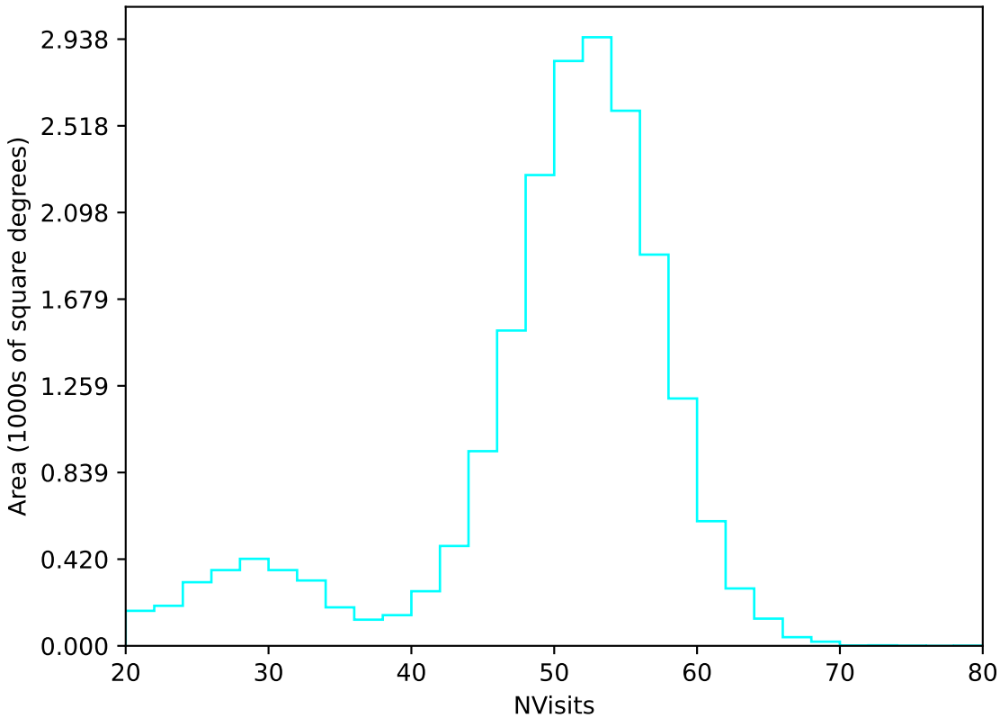
too_elab_r128_d3_ugrizy_v3.4_10yrs All sky u band: NVisits
