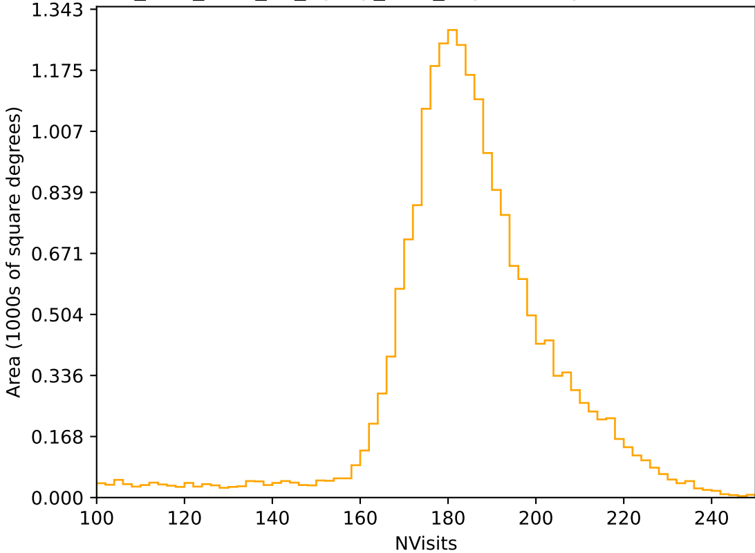
too_elab_r128_d3_ugrizy_v3.4_10yrs All sky r band: NVisits
