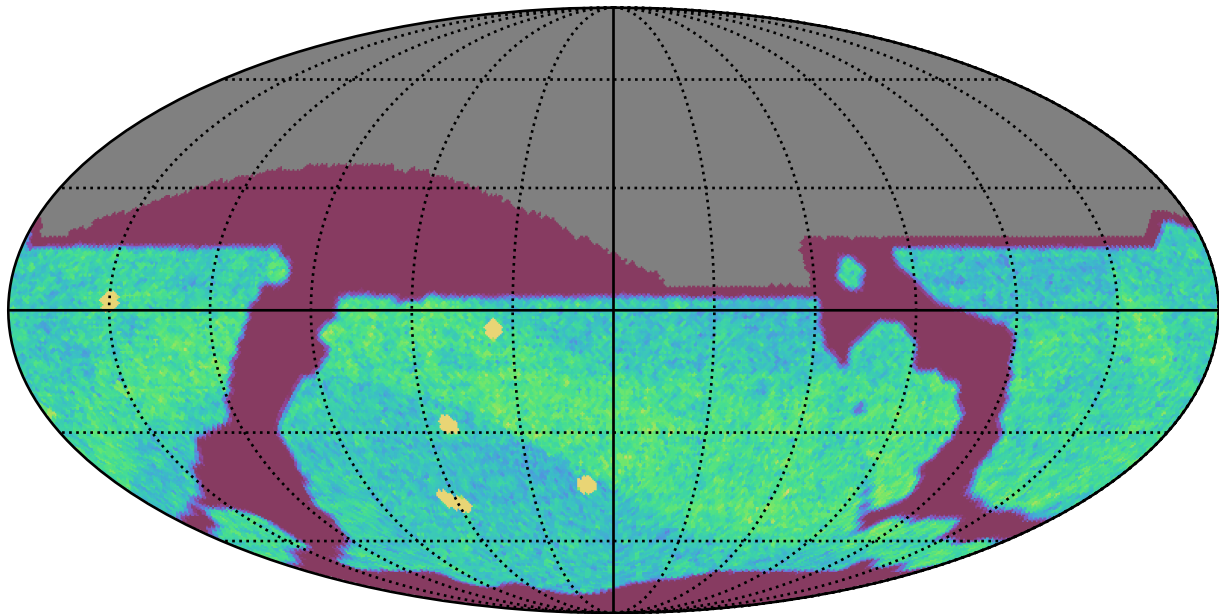
too_elab_r128_d3_ugrizy_v3.4_10yrs All sky i band: NVisits
