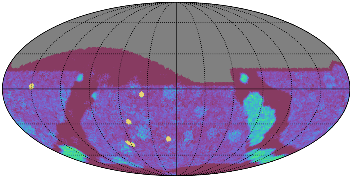
too_elab_r128_d3_ugrizy_v3.4_10yrs All sky g band: NVisits
