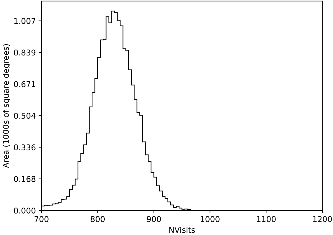
too_elab_r128_d3_ugrizy_v3.4_10yrs All sky all bands: NVisits
