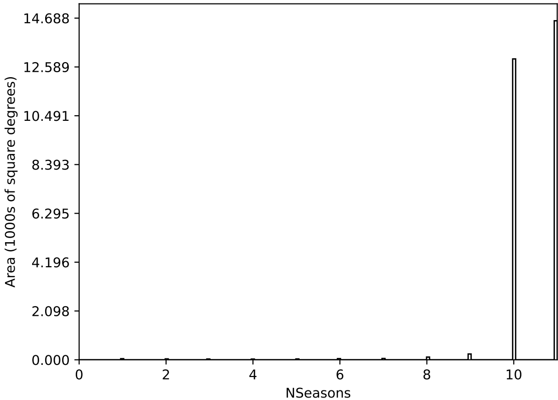
too_elab_r128_d3_ugrizy_v3.4_10yrs All sky all bands: NSeasons
