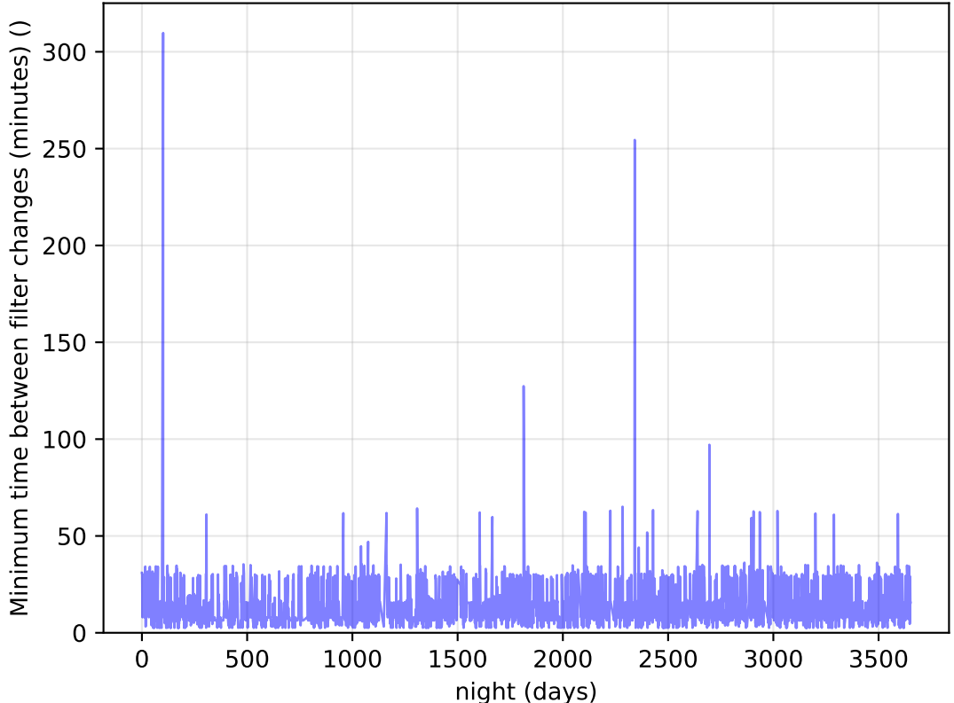
too_elab_r128_d3_ugrizy_v3.4_10yrs Per Night: Minimum time between filter changes (minutes)
