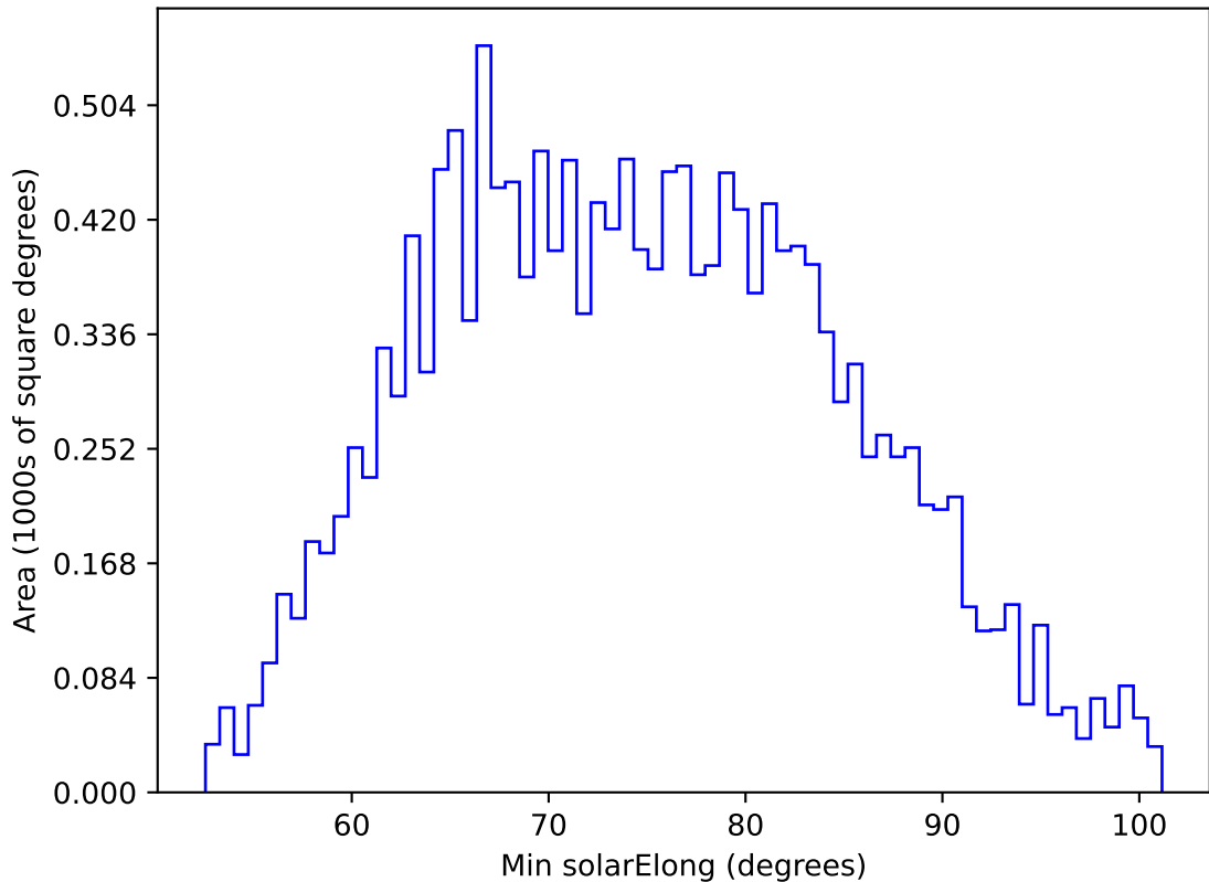
too_elab_r128_d3_ugrizy_v3.4_10yrs WFD u band: Min solarElong
