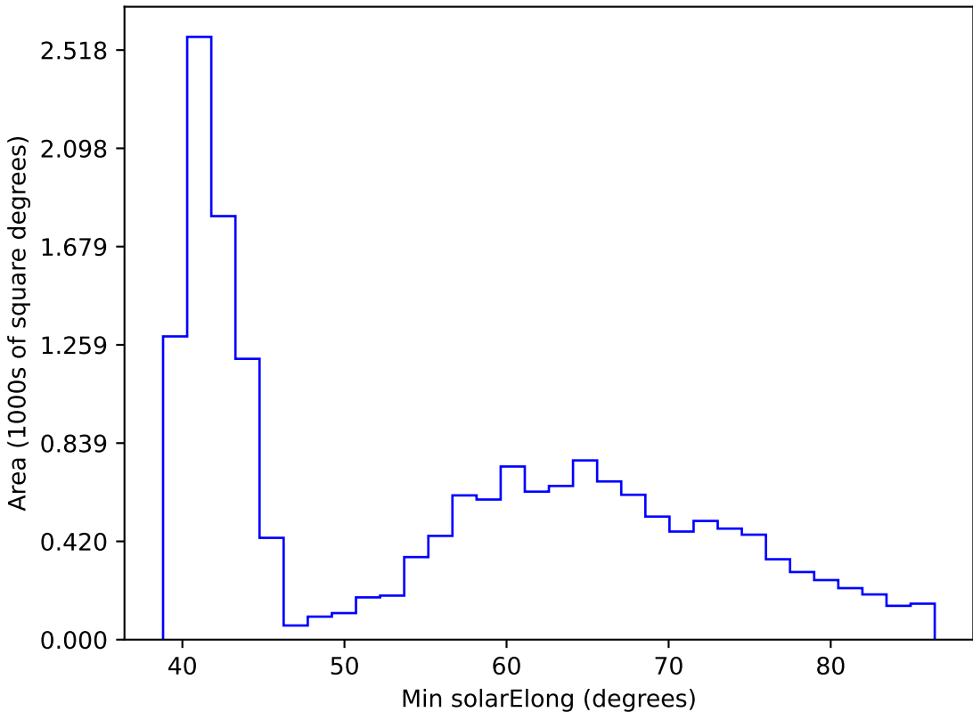
too_elab_r128_d3_ugrizy_v3.4_10yrs WFD r band: Min solarElong
