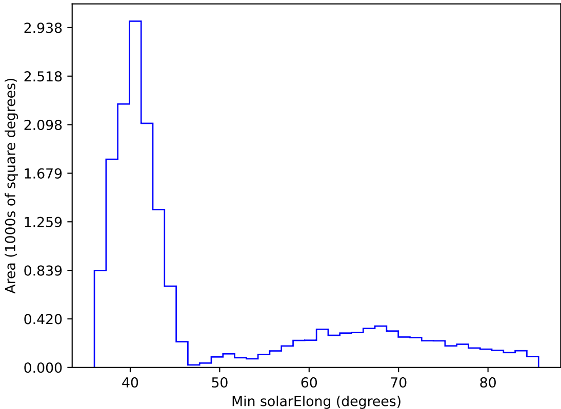
too_elab_r128_d3_ugrizy_v3.4_10yrs WFD i band: Min solarElong
