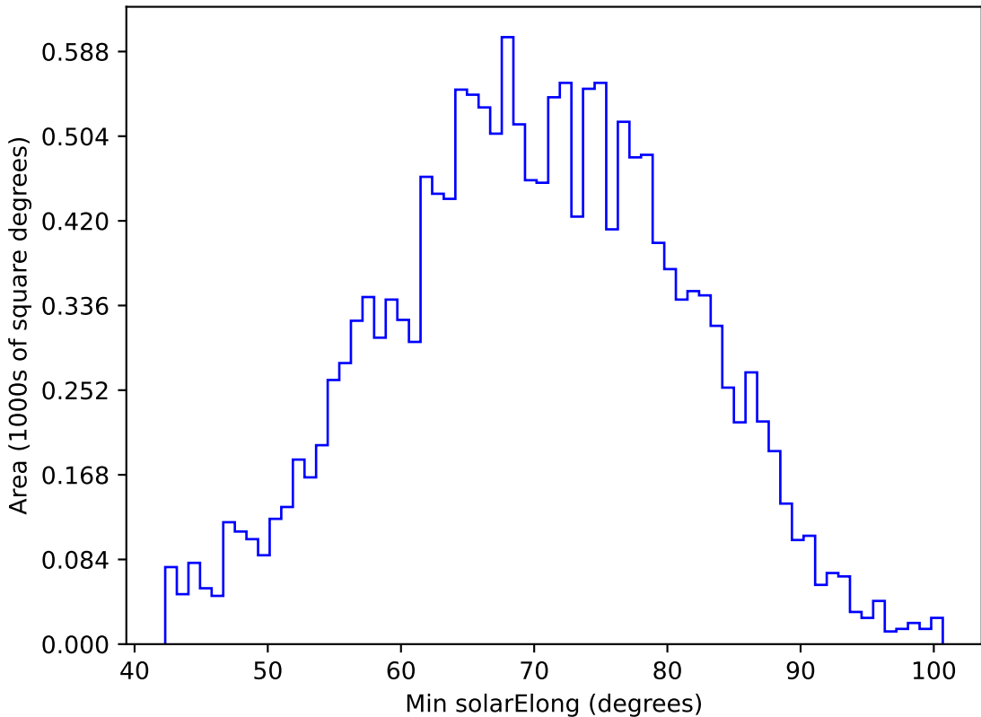
too_elab_r128_d3_ugrizy_v3.4_10yrs WFD g band: Min solarElong
