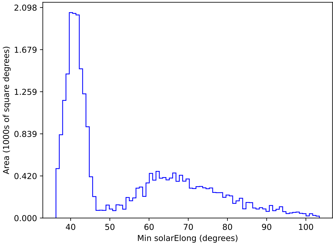
too_elab_r128_d3_ugrizy_v3.4_10yrs All sky z band: Min solarElong
