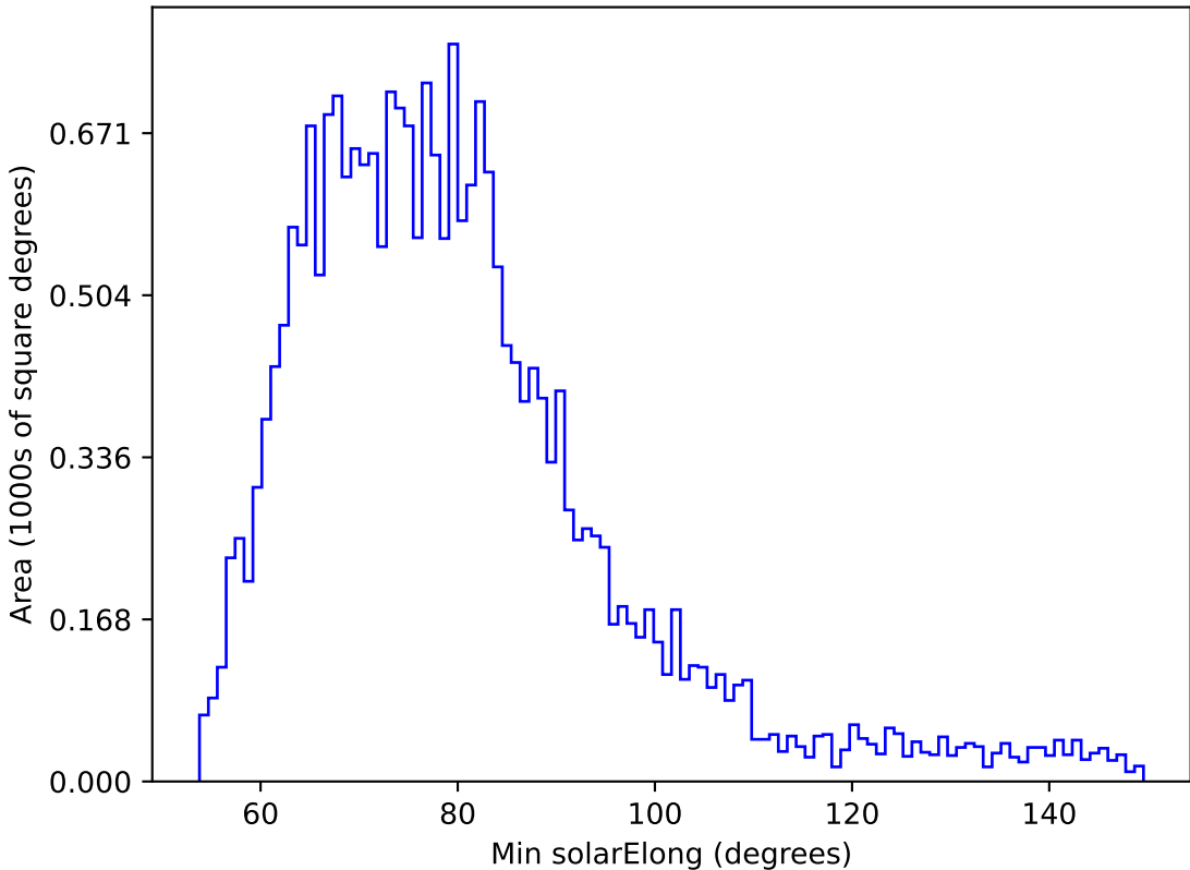
too_elab_r128_d3_ugrizy_v3.4_10yrs All sky u band: Min solarElong
