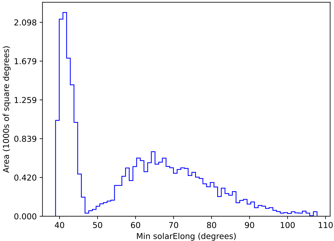
too_elab_r128_d3_ugrizy_v3.4_10yrs All sky r band: Min solarElong
