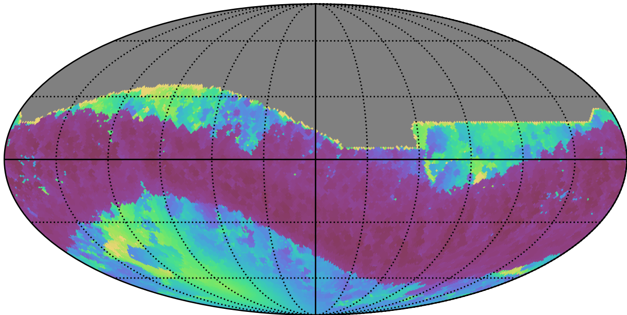
too_elab_r128_d3_ugrizy_v3.4_10yrs All sky i band: Min solarElong
