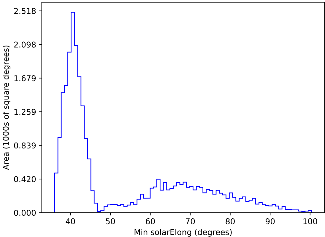
too_elab_r128_d3_ugrizy_v3.4_10yrs All sky i band: Min solarElong
