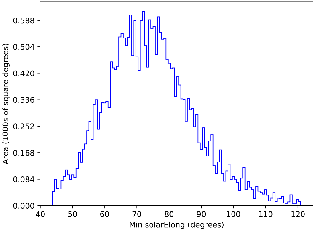
too_elab_r128_d3_ugrizy_v3.4_10yrs All sky g band: Min solarElong
