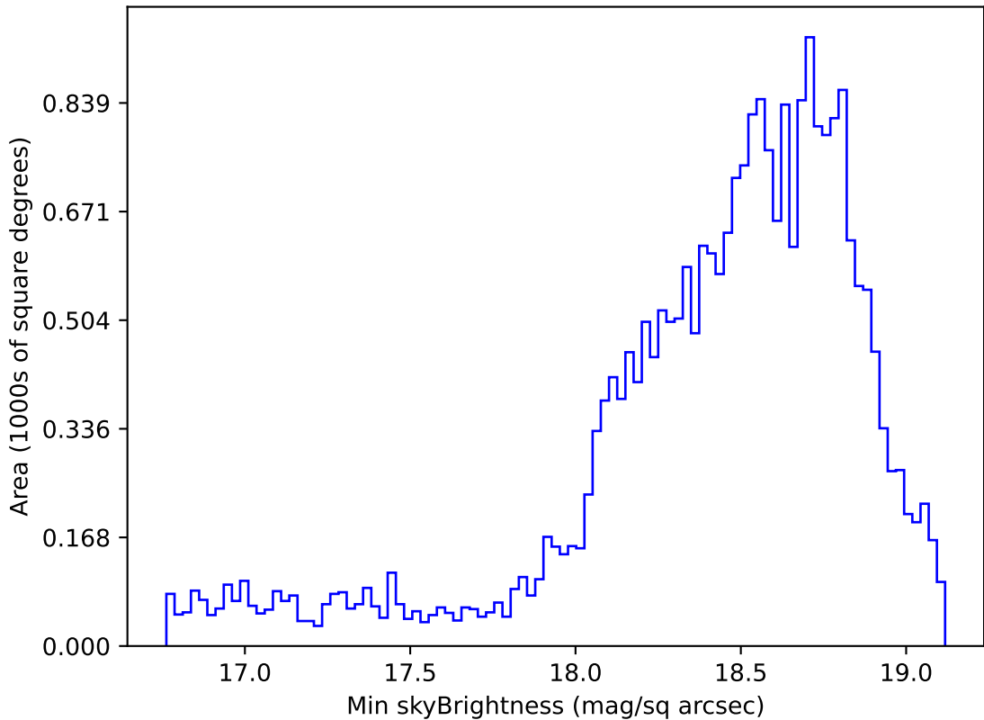
too_elab_r128_d3_ugrizy_v3.4_10yrs Yr 1 z band: Min skyBrightness
