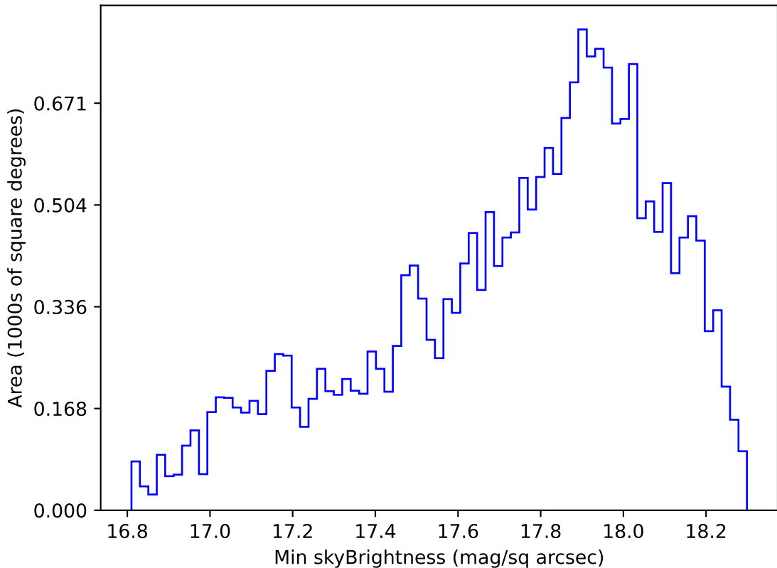
too_elab_r128_d3_ugrizy_v3.4_10yrs Yr 1 y band: Min skyBrightness
