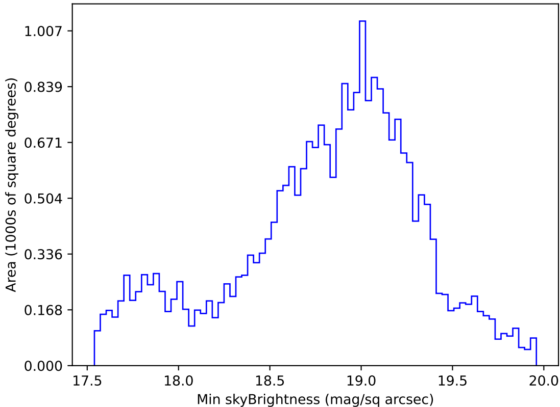
too_elab_r128_d3_ugrizy_v3.4_10yrs Yr 1 i band: Min skyBrightness
