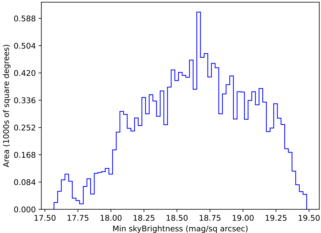
too_elab_r128_d3_ugrizy_v3.4_10yrs WFD r band: Min skyBrightness
