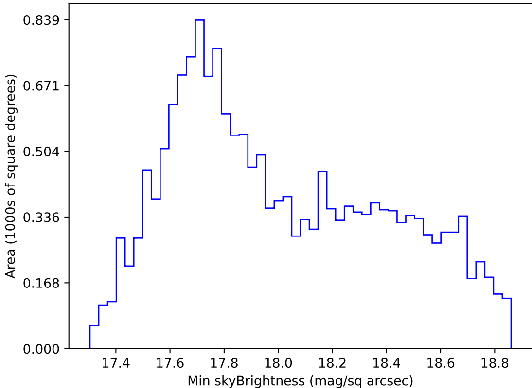
too_elab_r128_d3_ugrizy_v3.4_10yrs WFD i band: Min skyBrightness
