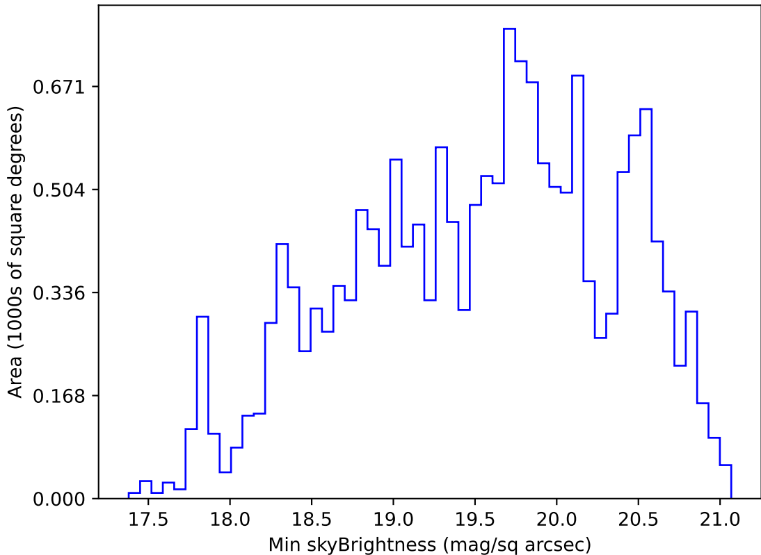
too_elab_r128_d3_ugrizy_v3.4_10yrs WFD g band: Min skyBrightness
