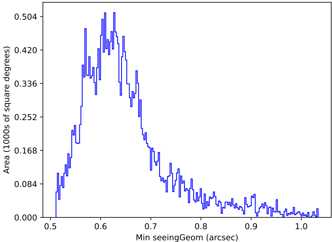
too_elab_r128_d3_ugrizy_v3.4_10yrs Yr 1 z band: Min seeingGeom
