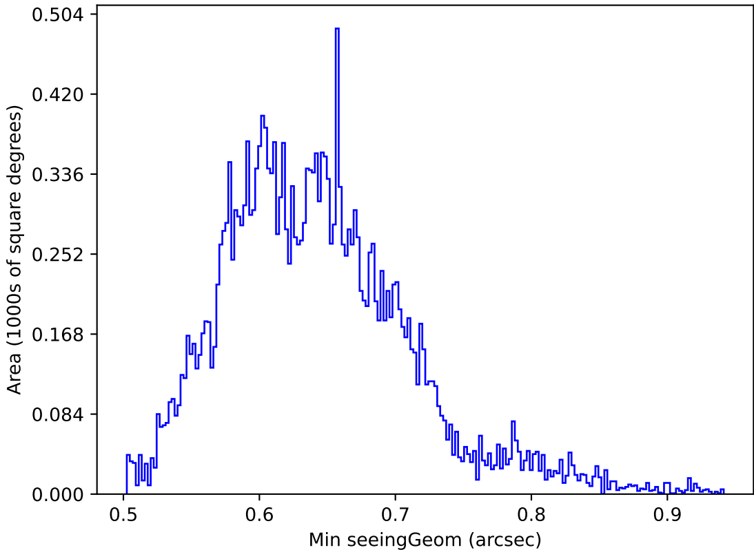
too_elab_r128_d3_ugrizy_v3.4_10yrs Yr 1 y band: Min seeingGeom
