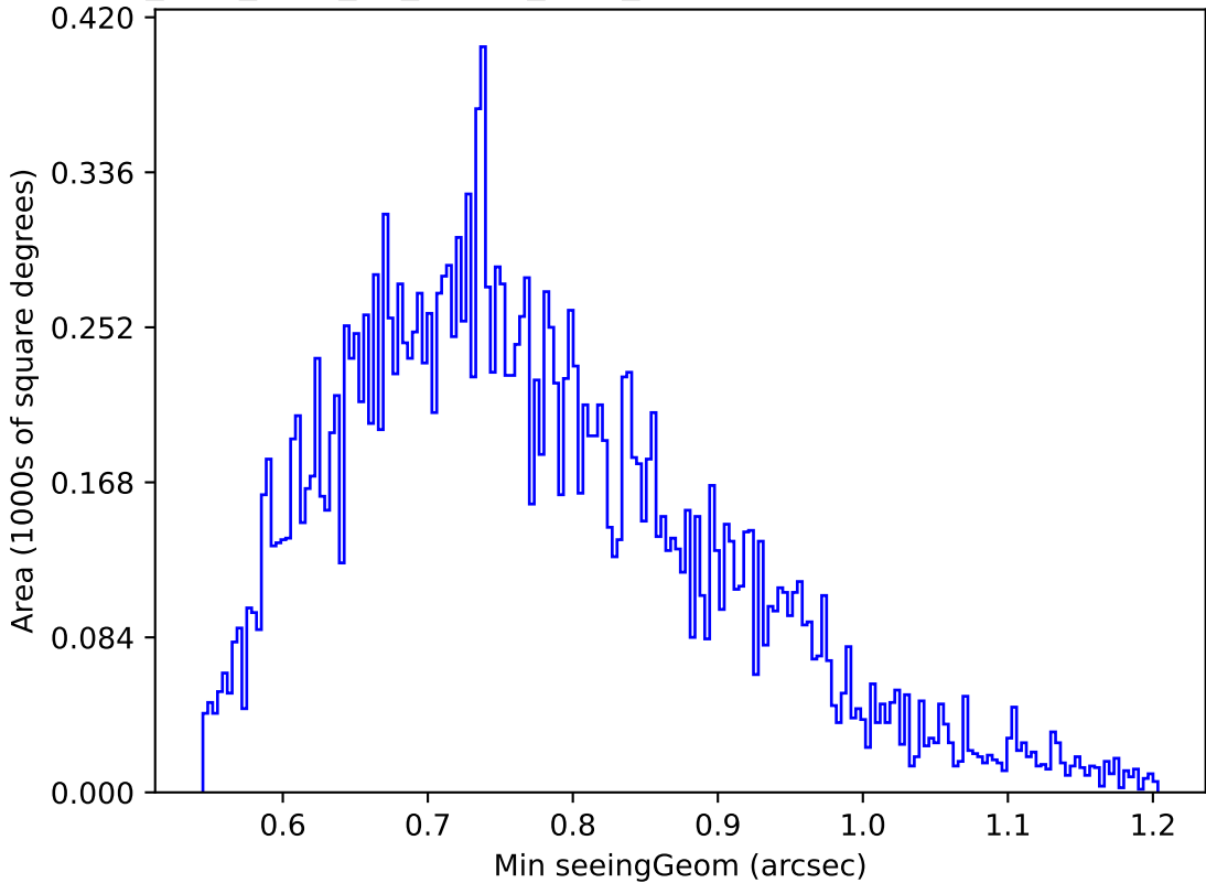
too_elab_r128_d3_ugrizy_v3.4_10yrs Yr 1 u band: Min seeingGeom
