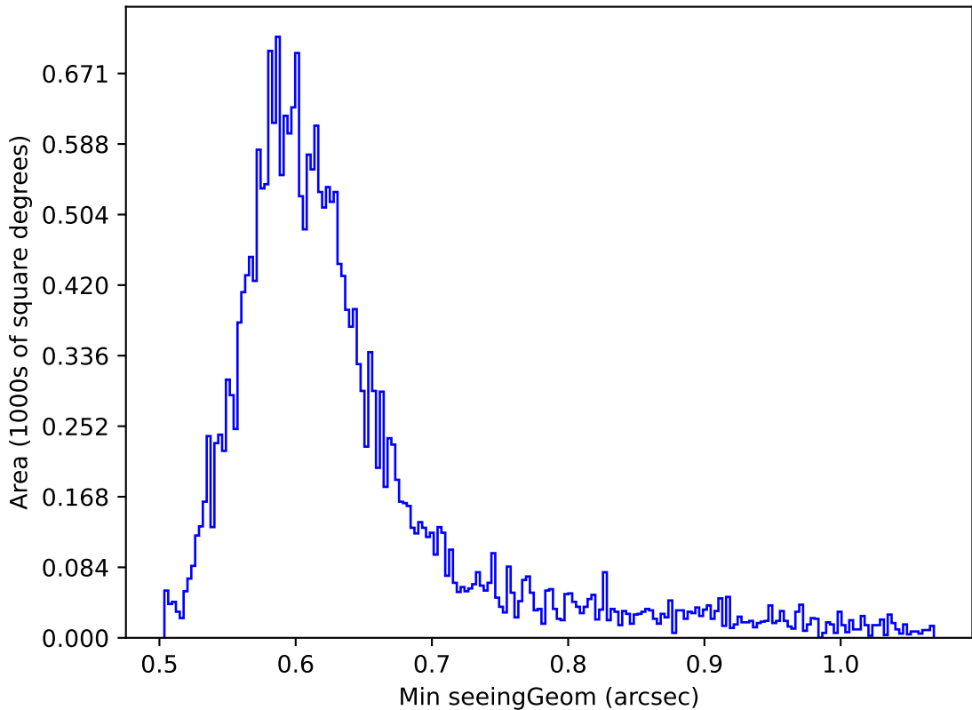
too_elab_r128_d3_ugrizy_v3.4_10yrs Yr 1 i band: Min seeingGeom
