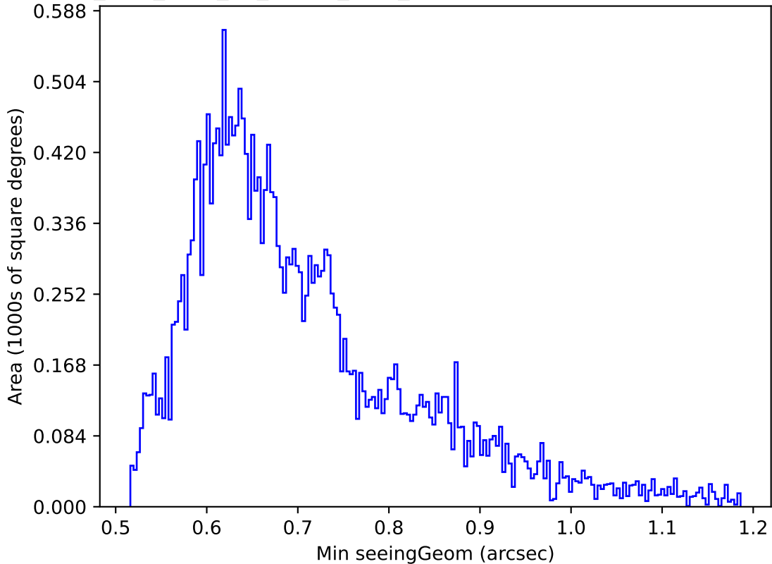
too_elab_r128_d3_ugrizy_v3.4_10yrs Yr 1 g band: Min seeingGeom
