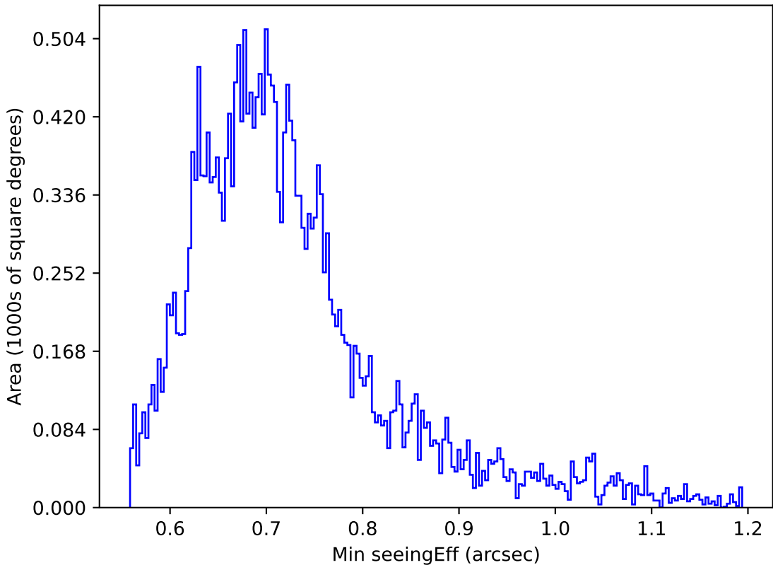
too_elab_r128_d3_ugrizy_v3.4_10yrs Yr 1 z band: Min seeingEff
