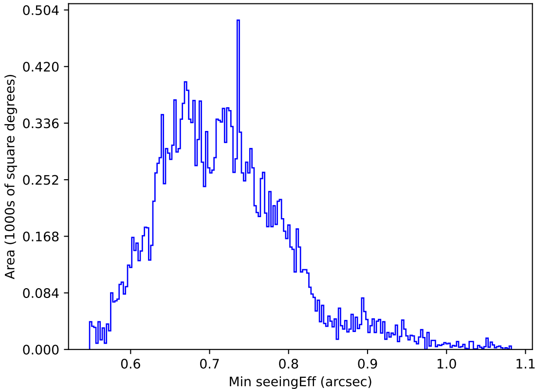
too_elab_r128_d3_ugrizy_v3.4_10yrs Yr 1 y band: Min seeingEff
