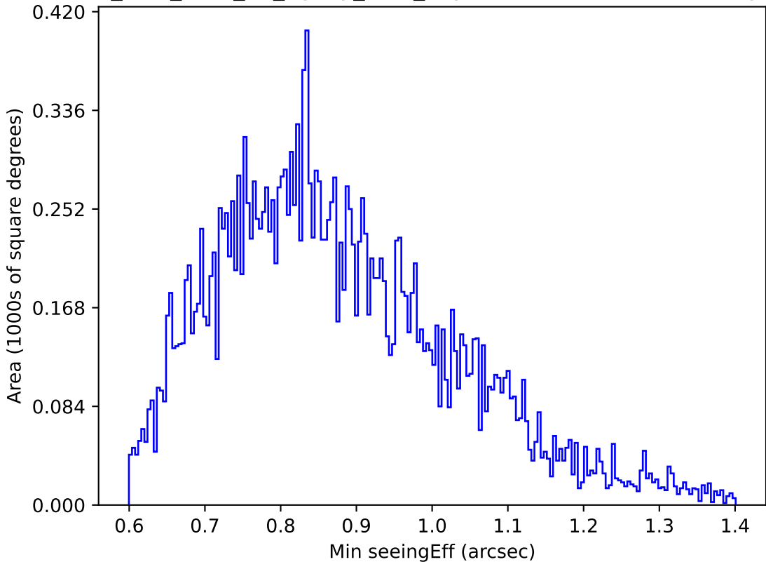
too_elab_r128_d3_ugrizy_v3.4_10yrs Yr 1 u band: Min seeingEff
