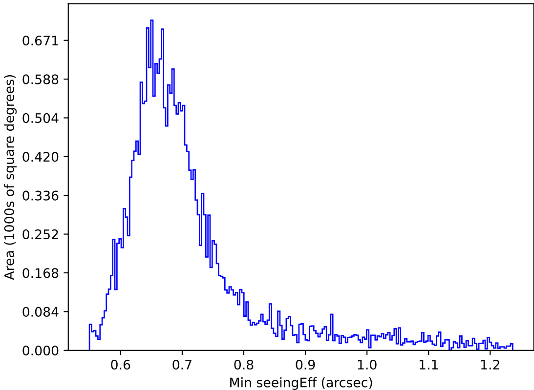
too_elab_r128_d3_ugrizy_v3.4_10yrs Yr 1 i band: Min seeingEff
