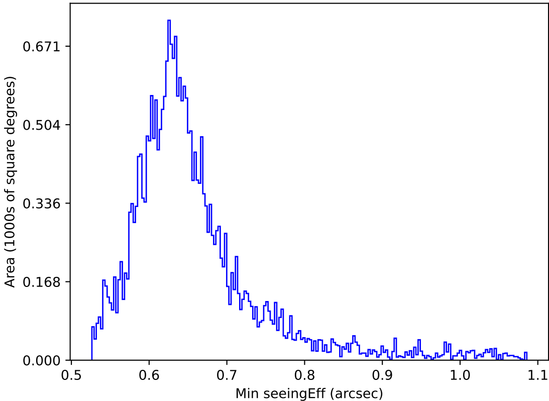
too_elab_r128_d3_ugrizy_v3.4_10yrs Yr 1 all bands: Min seeingEff
