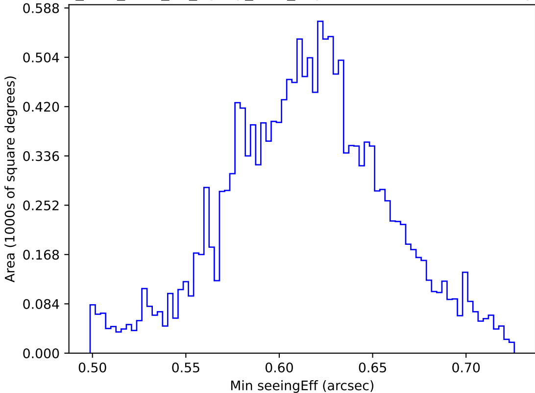
too_elab_r128_d3_ugrizy_v3.4_10yrs WFD z band: Min seeingEff
