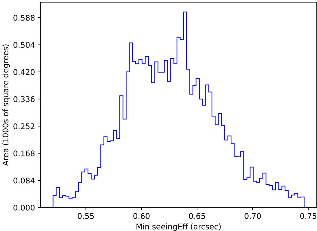
too_elab_r128_d3_ugrizy_v3.4_10yrs WFD y band: Min seeingEff
