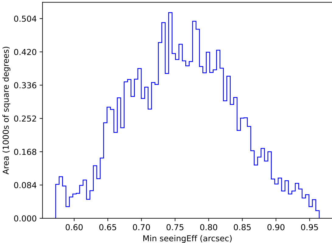
too_elab_r128_d3_ugrizy_v3.4_10yrs WFD u band: Min seeingEff
