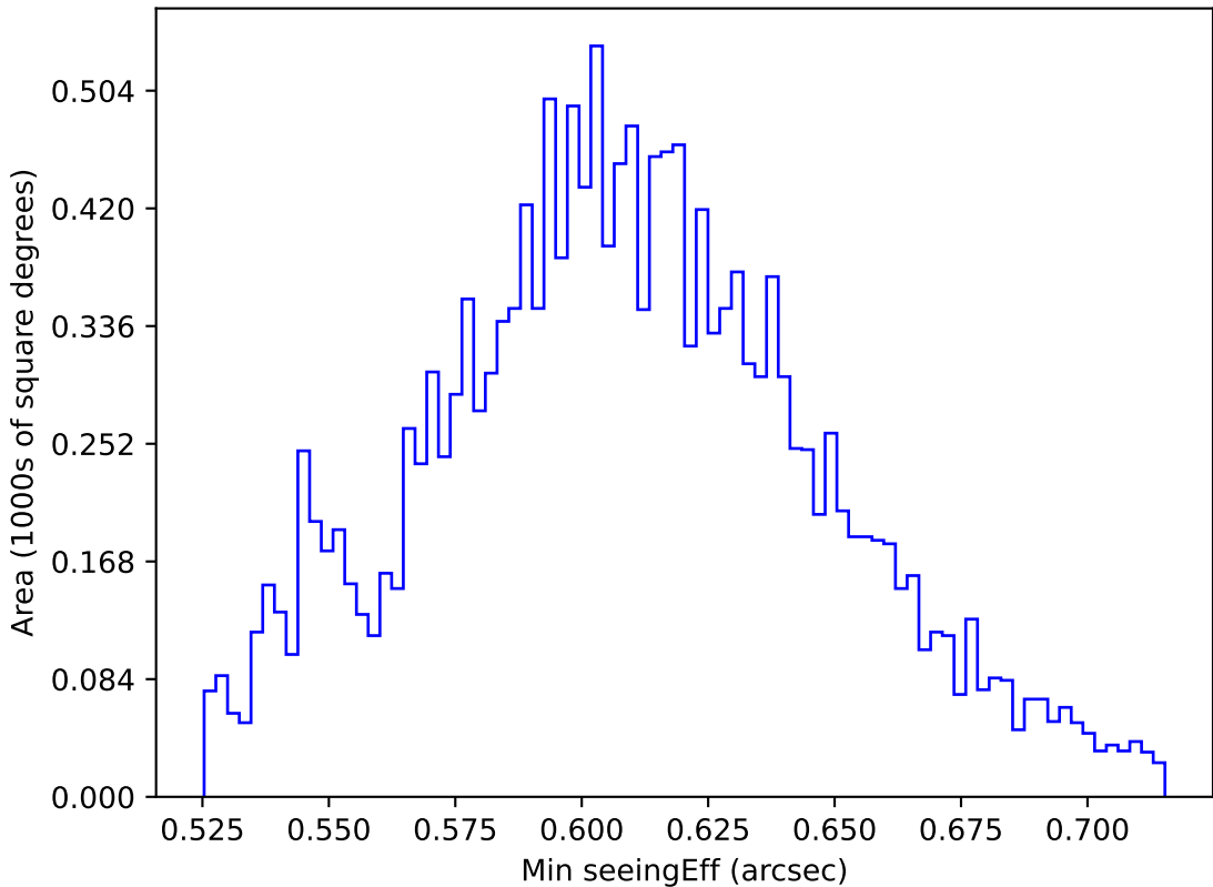
too_elab_r128_d3_ugrizy_v3.4_10yrs WFD i band: Min seeingEff
