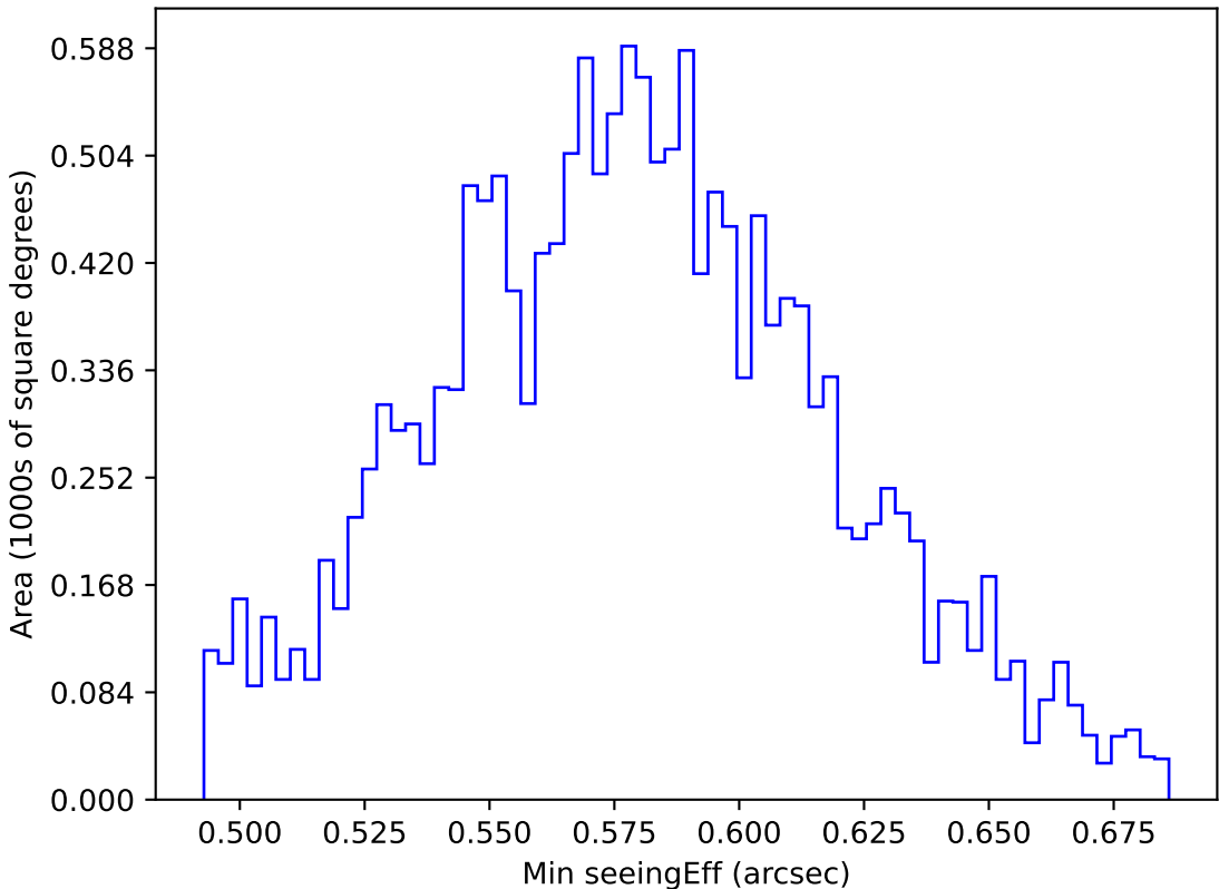
too_elab_r128_d3_ugrizy_v3.4_10yrs WFD all bands: Min seeingEff
